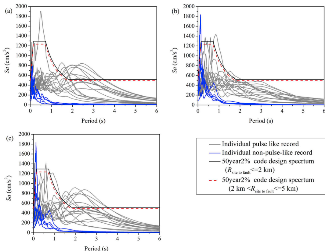
Fig. 17. Comparison between the acceleration spectrum (damping ratio = 5%) of near-field records observed in Hualien earthquake and the code design spectrum; (a),(b) and (c) represents the EW, NS components and the component rotated to the maximum pulse-like orientation respectively.
