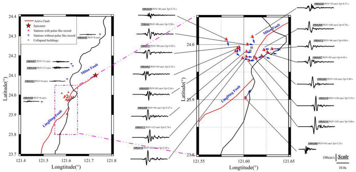
Fig. 4. The velocity time histories were rotated in the maximum pulse-like orientations area regarding the stations with/without velocity pulses in the studied near-field. The epicenter, fault and four collapsed buildings in Hualien city were illustrated in the map. The maximum pulse orientations were presented using blue arrows for the stations with identified pulse-like velocities in Table 2. (For interpretation of the references to colour in this figure legend, the reader is referred to the Web version of this article.)
