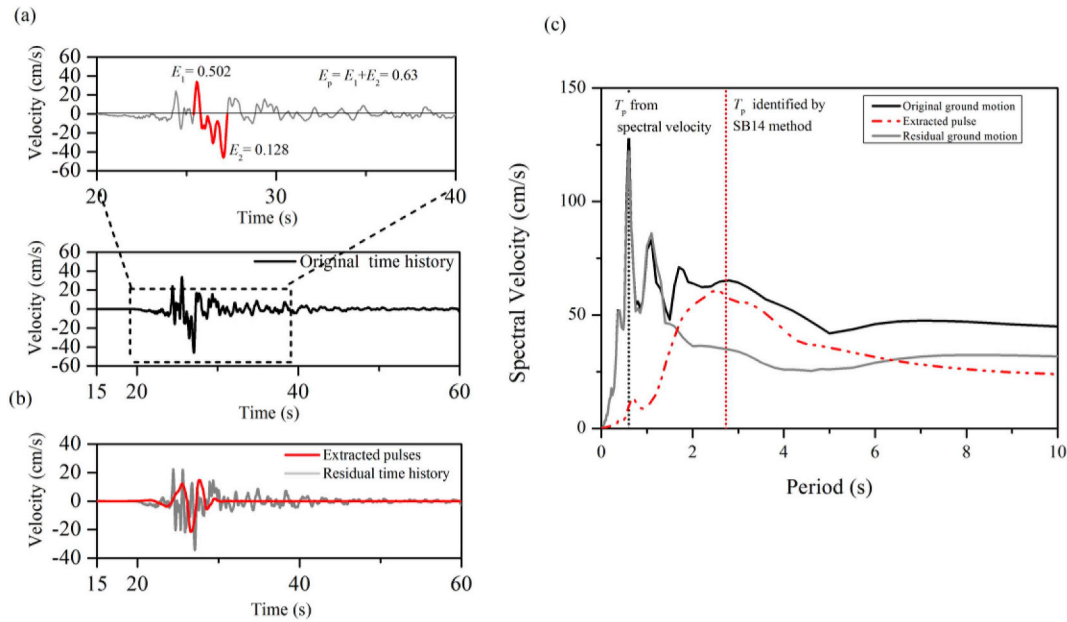
Fig. 7. (a) Significant velocity half-cycles and energy ratios computed using method in Zhai et al(2018) [25][] for the HWA048 station; (b) The extracted velocity pulse computed using SB14 method and residual time histories (c) Velocity response spectrum of the original record, extracted pulses and the residual record, with labels noting the identified T_p values using wavelet algorithm and peak of velocity spectrum.
